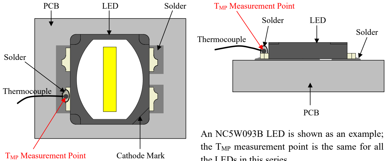
Figure 1. T MP Measurement Point
