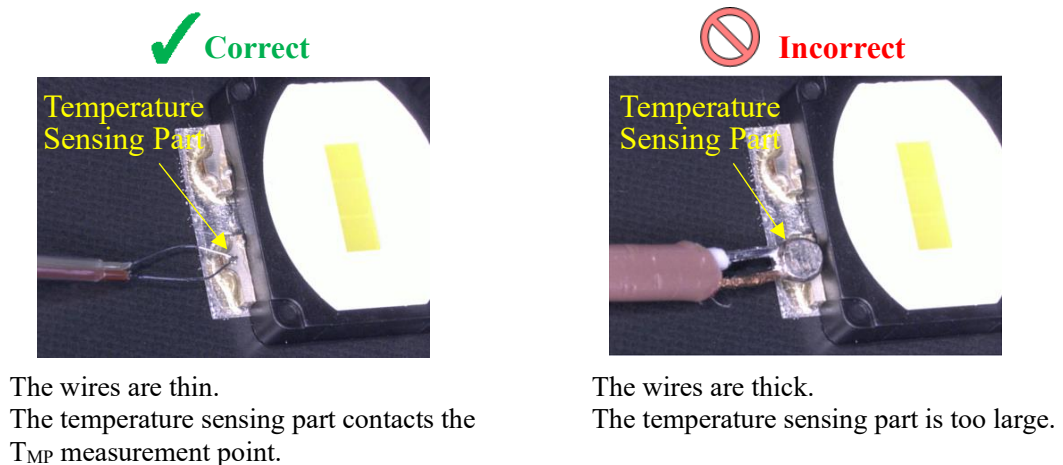
Figure 2. Examples of Correct/Incorrect Thermocouples (Before soldering to the die heatsink)
