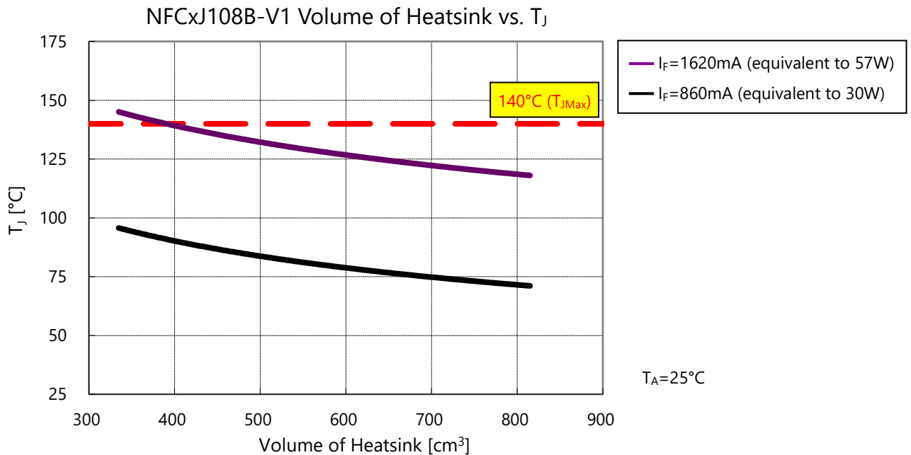
Figure 6. Evaluation Result for the NFCxJ108B-V1 COB LEDs
