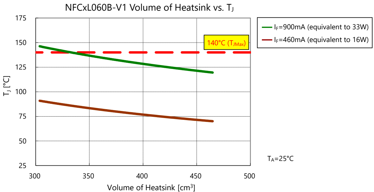
Figure 5. Evaluation Result for the NFCxL060B-V1 COB LEDs
