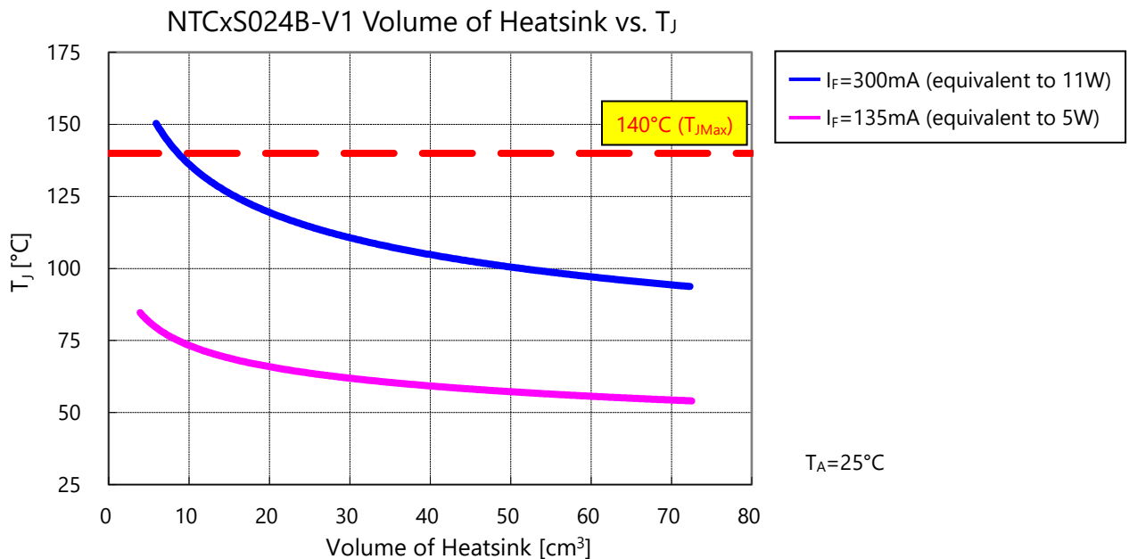
Figure 3. Evaluation Result for the NTCxS024B-V1 COB LEDs
