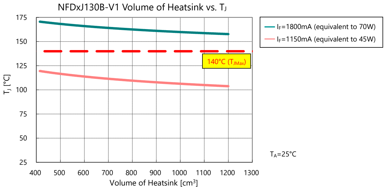
Figure 7. Evaluation Result for the NFDxJ130B-V1 COB LEDs
