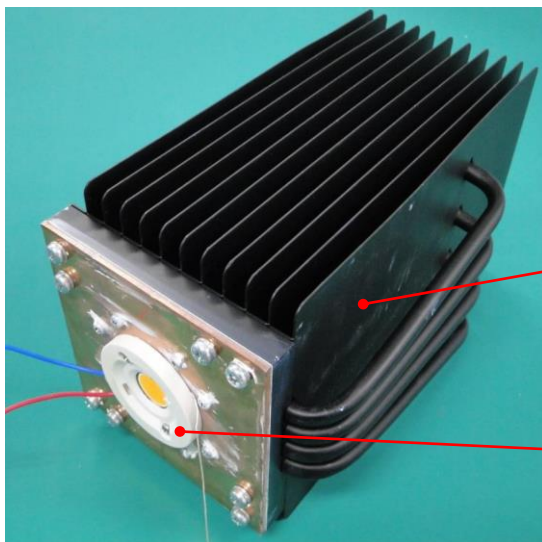
Figure 8. Conditions of the evaluation using a heatsink with heat pipes
