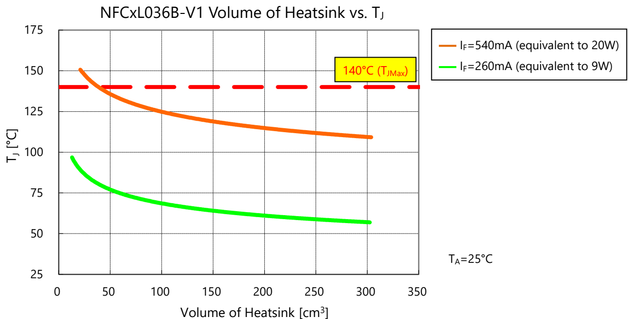
Figure 4. Evaluation Result for the NFCxL036B-V1 COB LEDs
