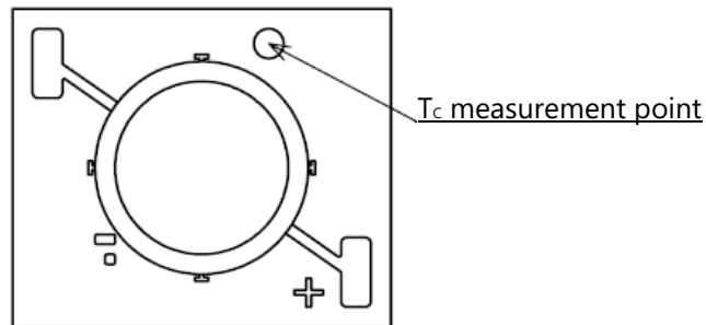
Figure 2. Position of the T_c measurement point
