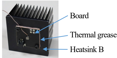
Picture 3. Evaluated light source 4-2
