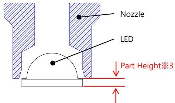
Figure 3. Cross-sectional view of a nozzle when transporting an Nichia 119/219 series LEDs
