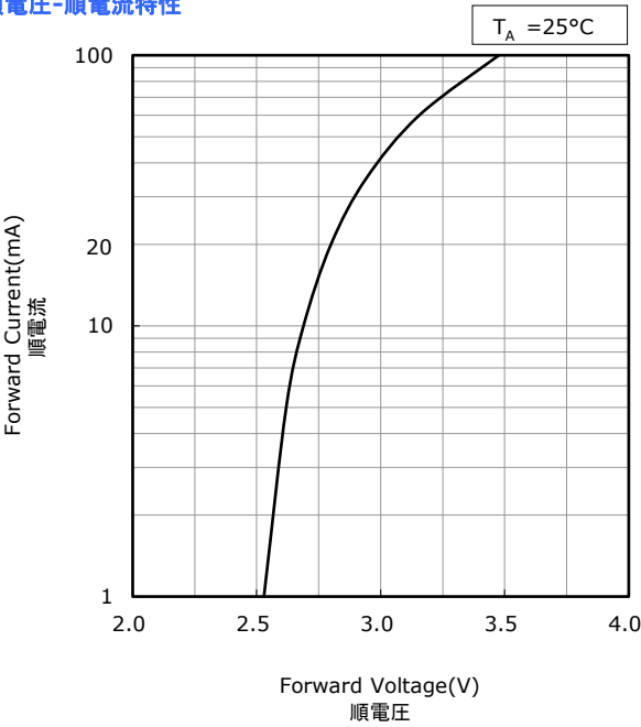
Forward Voltage vs Forward Current 順電圧-順電流特性
