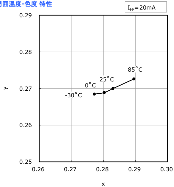
Ambient Temperature vs Chromaticity Coordinate
