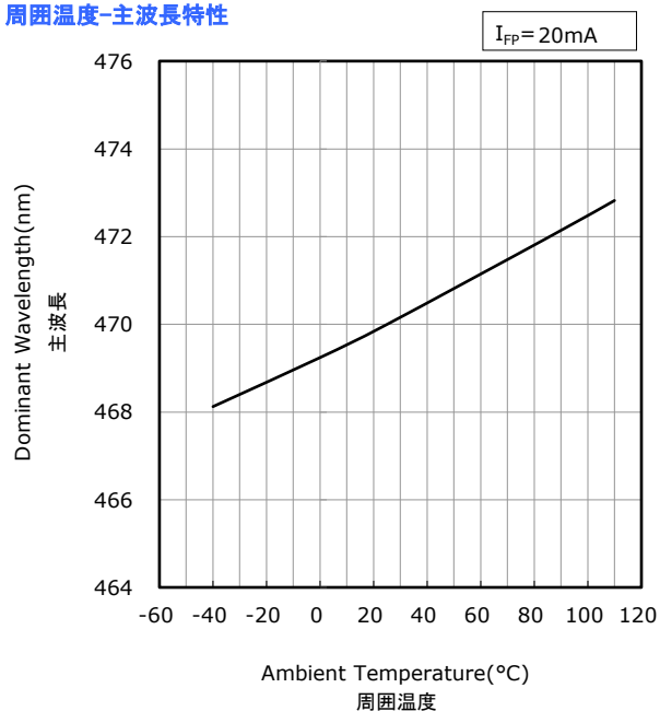
Ambient Temperature vs Dominant Wavelength
