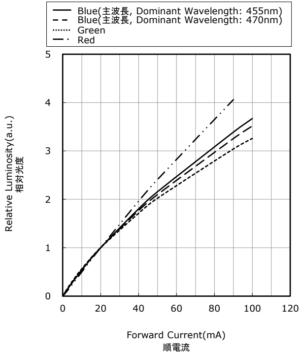
Forward Current vs Relative Luminosity
