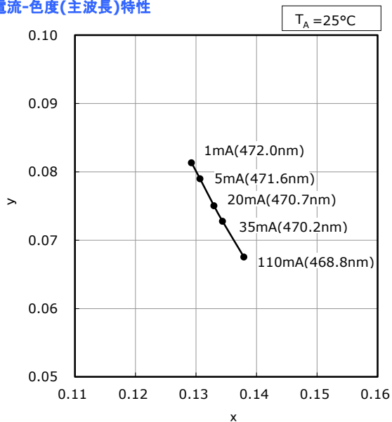
Forward Current vs Chromaticity Coordinate( \lambda_d )
