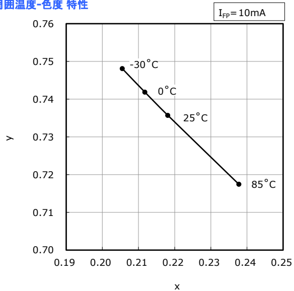
Ambient Temperature vs Chromaticity Coordinate
