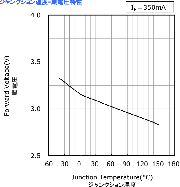
Junction Temperature vs Forward Voltage
