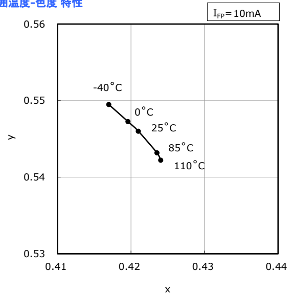
Ambient Temperature vs Chromaticity Coordinate
