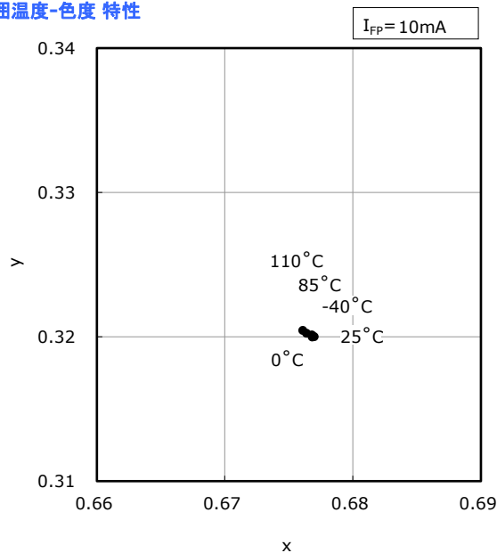
Ambient Temperature vs Chromaticity Coordinate
