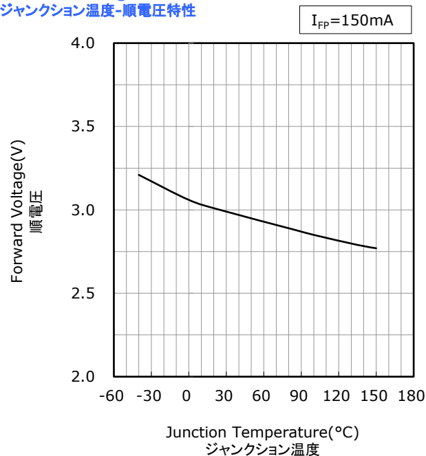
Junction Temperature vs Forward Voltage
