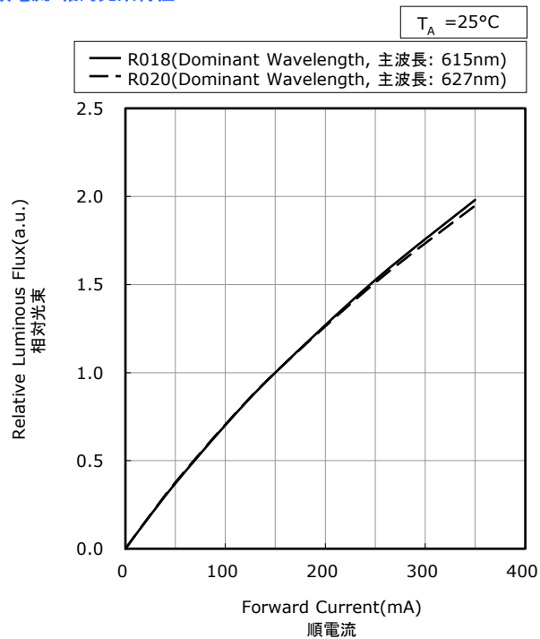
Forward Current vs Relative Luminous Flux 順電流-相対光束特性
