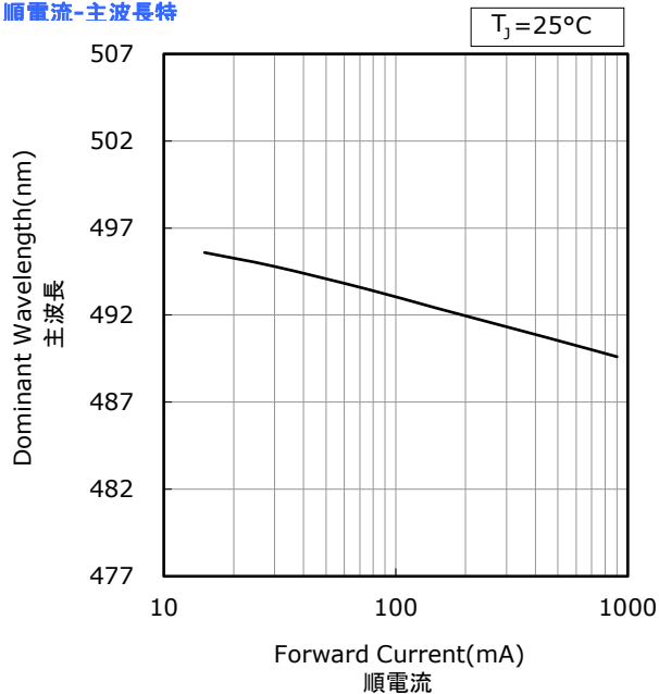
Forward Current vs Dominant Wavelength 順電流-主波長特
