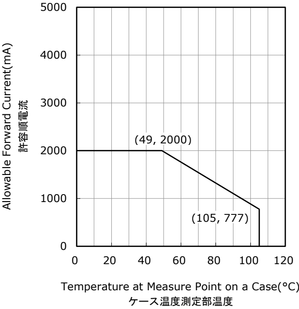
Temperature at Measure Point on a Case vs Allowable Forward Current ケース温度測定部温度-許容順電流特性
