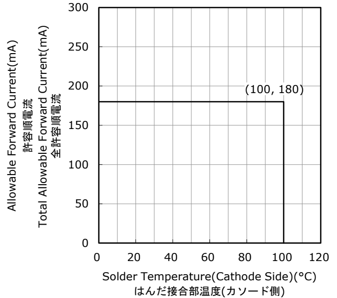
Solder Temperature(Cathode Side) vs Allowable Forward Current, Total Allowable Forward Current はんだ接合部温度(カソード側)-許容順電流、全許容順電流特性
