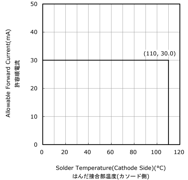
Solder Temperature(Cathode Side) vs Allowable Forward Current
