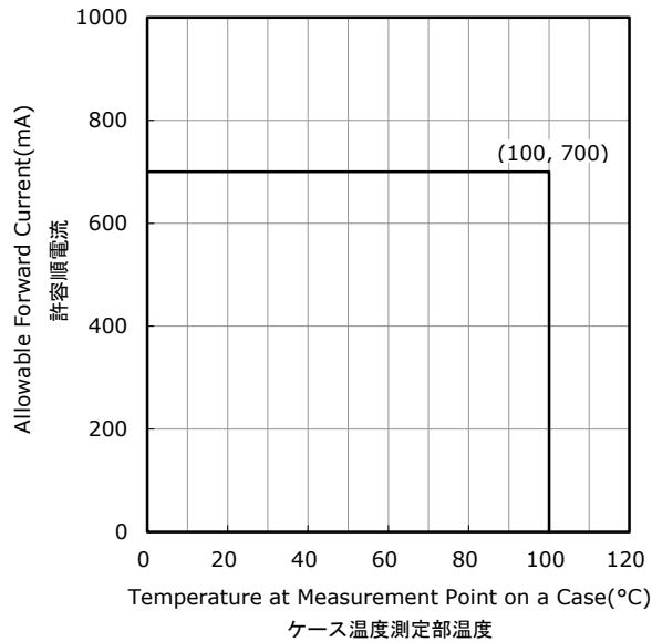
Temperature at Measurement Point on a Case vs Allowable Forward Current
