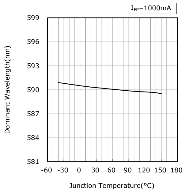
Junction Temperature vs Dominant Wavelength
