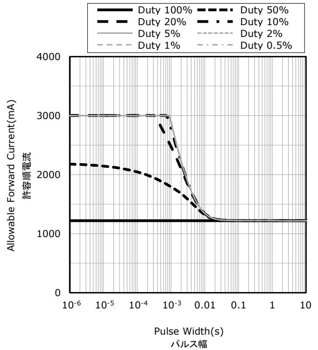
Pulse Width vs Allowable Forward Current
