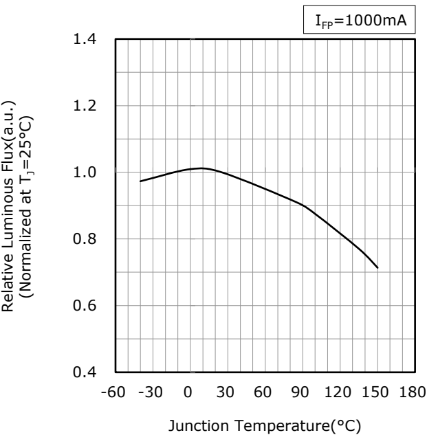
Junction Temperature vs Relative Luminous Flux
